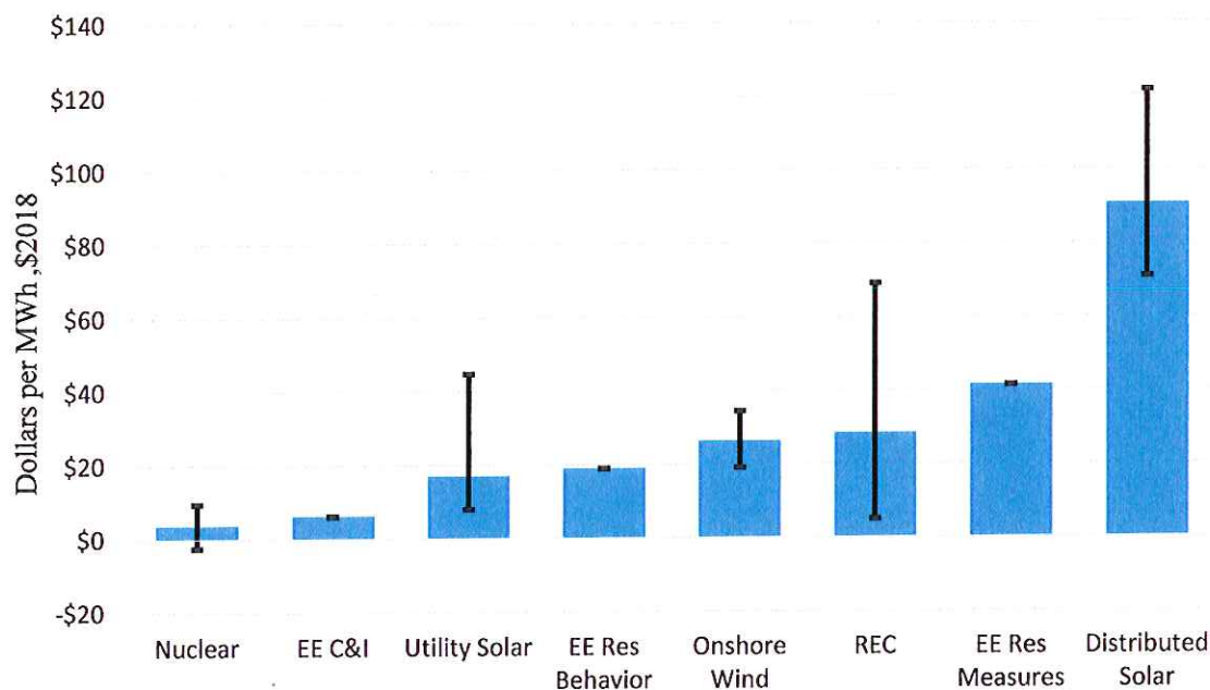
Figure 10: Levelized Net Cost per MWh in 2020, $2018
