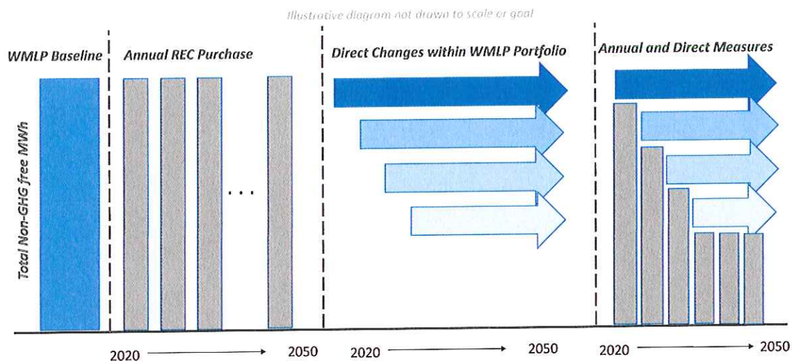
Figure 3: Illustrative and Representative Pathways to GHG Emission Goals
