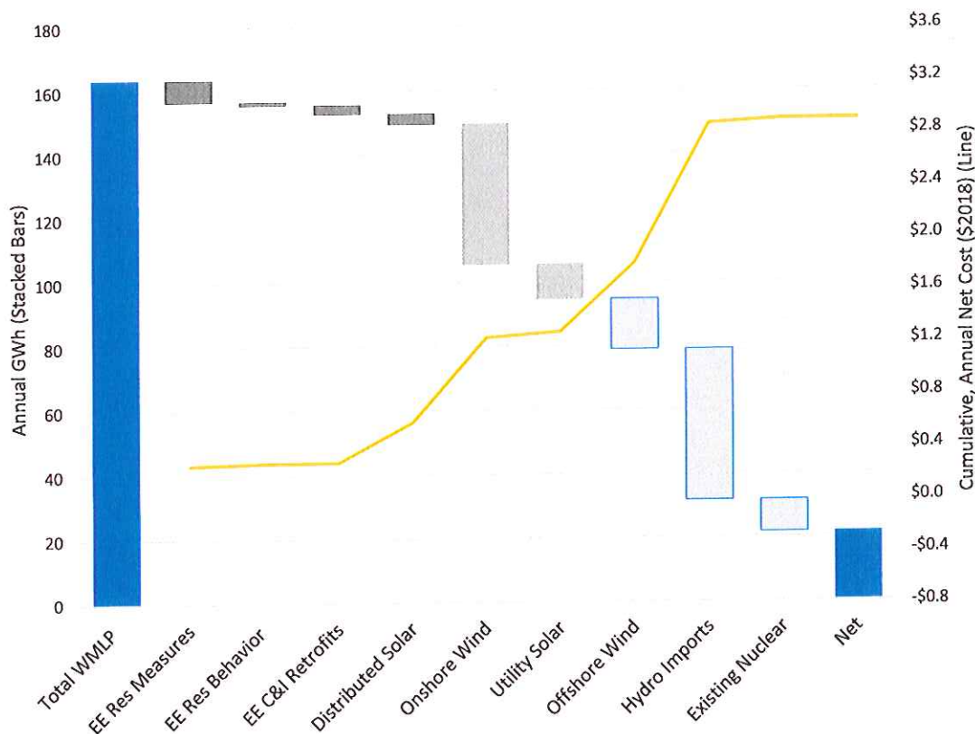
Executive Summary Figure 2: Cumulative Reductions and Net Costs in 2030 ($2018)
