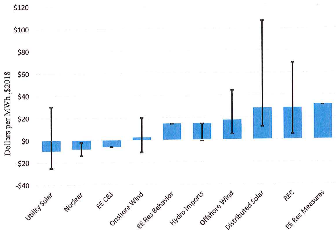
Executive Summary Figure 1: Levelized Net Cost Per MWh in 2030, $2018
