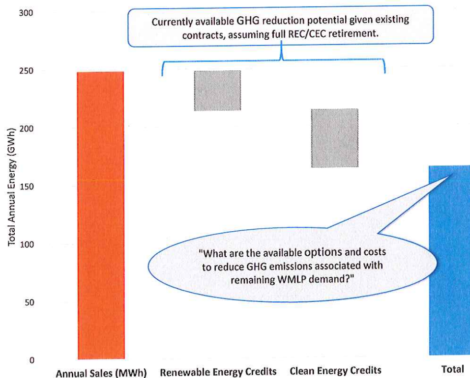
Figure 2: WMLP GHG Emission Free Portfolio (2022)
