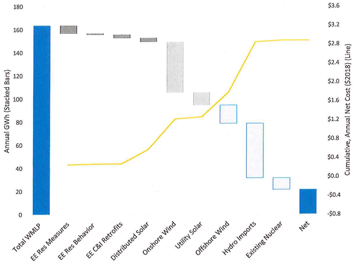
Figure 13: Cumulative GHG Emission Reductions and Net Costs in 2030 ($2018)
