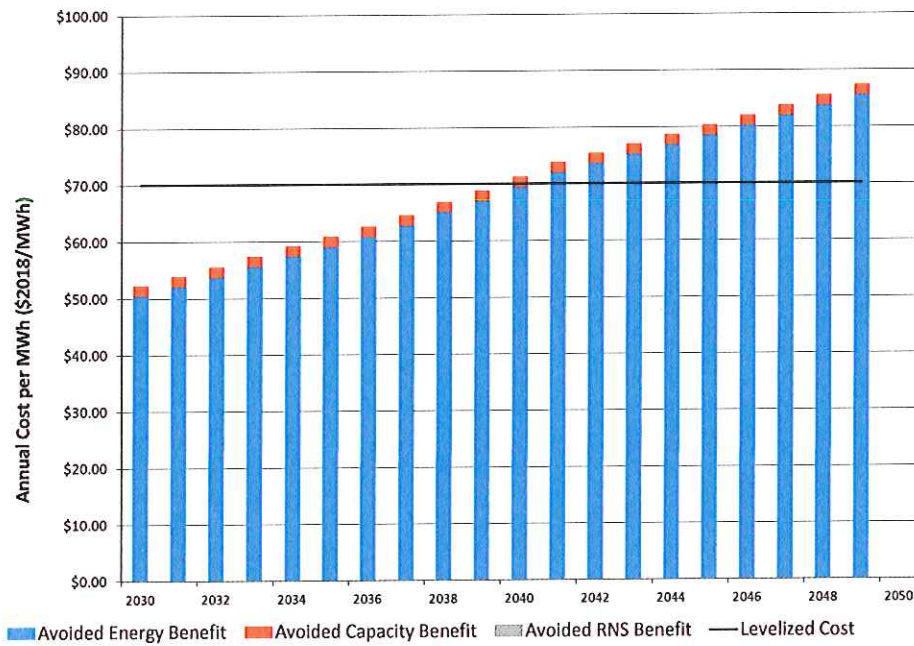
Figure 8: Annual Costs and Avoided Benefits ($/MWh), Onshore Wind, Installed 2030
