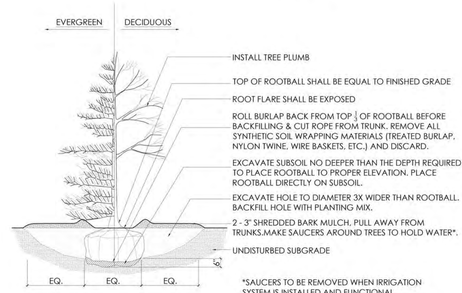
4 TREE PLANTING SCALE: 3/8" = 1'-0"
