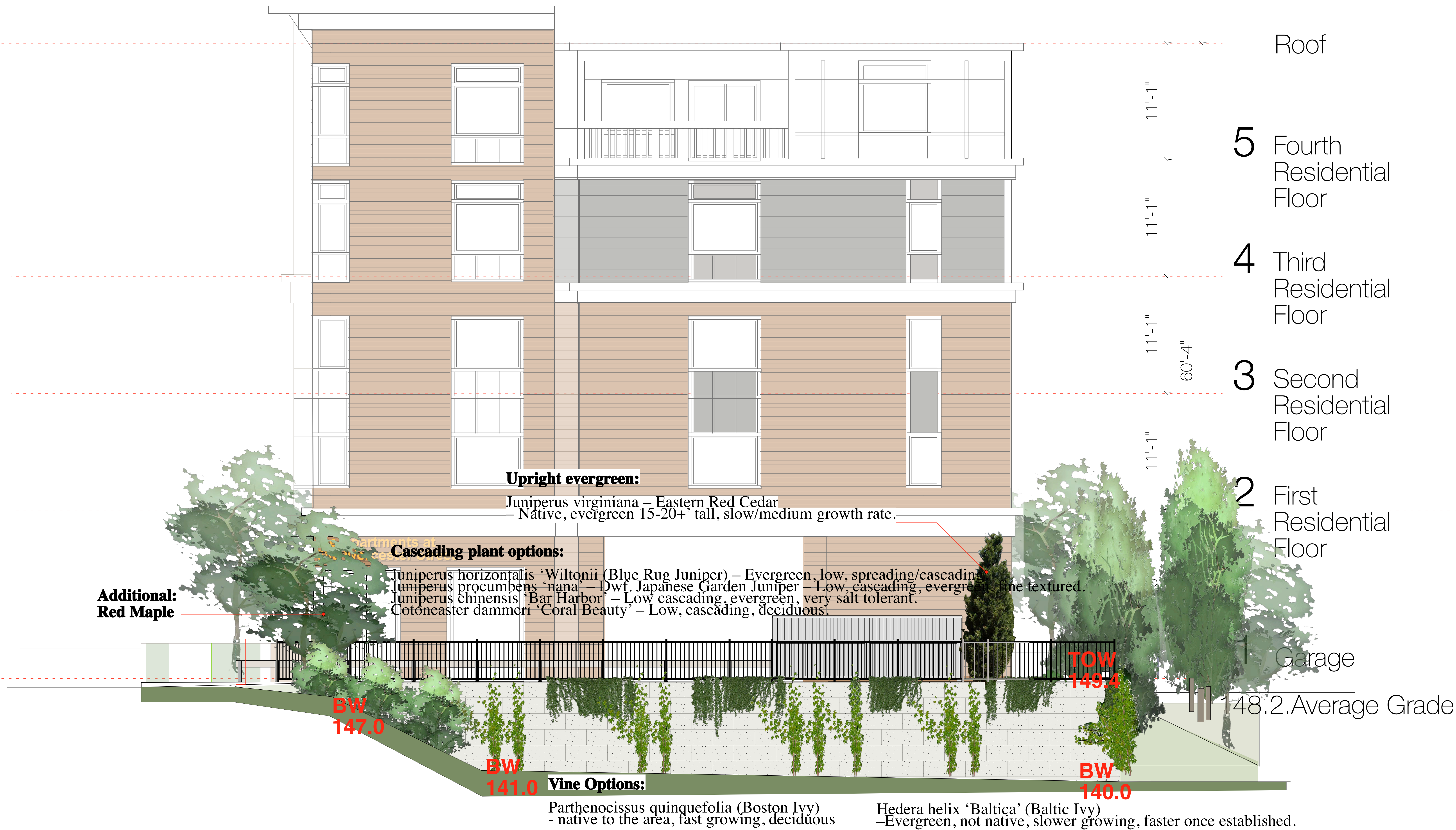
Retaining Wall at West Elevation
