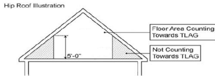
Figure 2. Attic TLAG Illustration – Hip Roof
