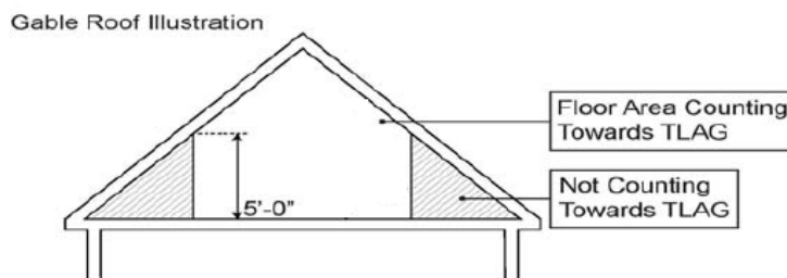
Figure 1. Attic TLAG Illustration – Gable Roof
