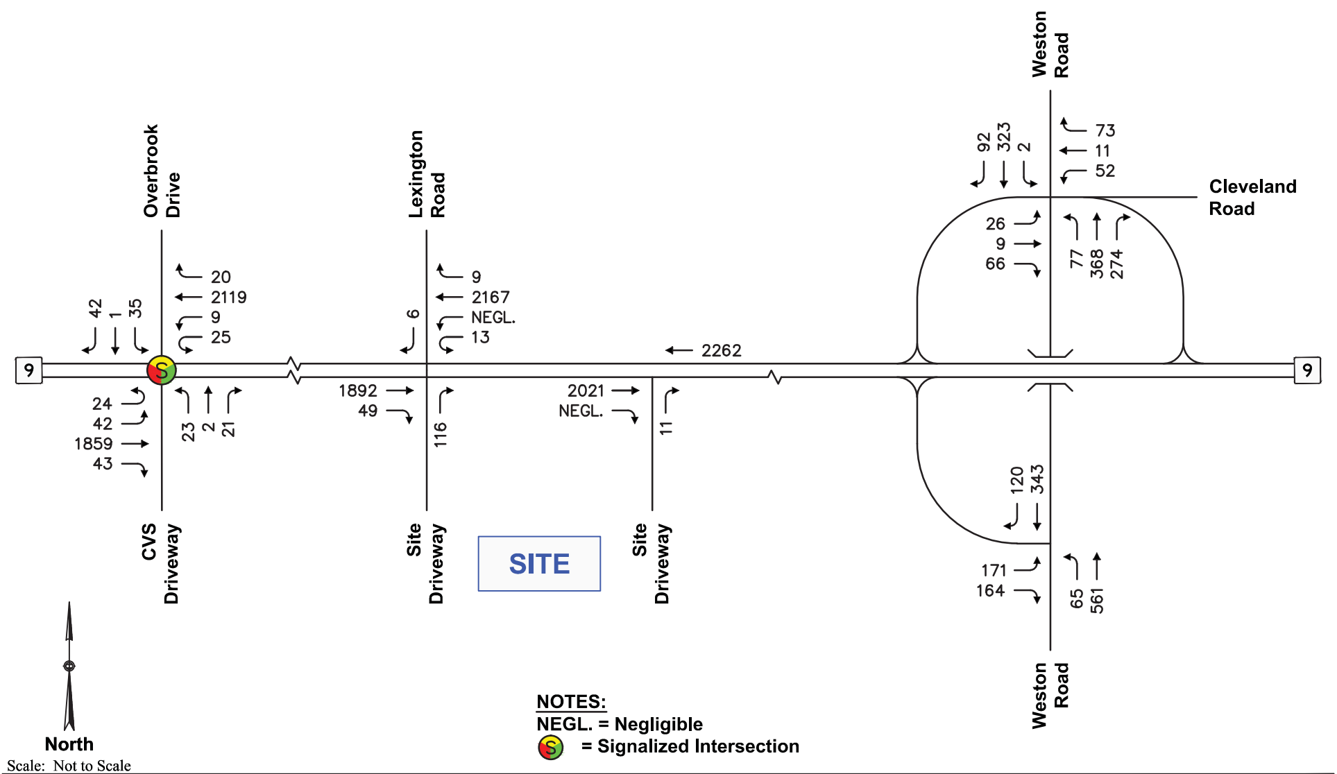
Figure 21 2024 Alternate Build Saturday Midday Peak Hour Traffic Volumes (Unsignalized Access Alternative)
