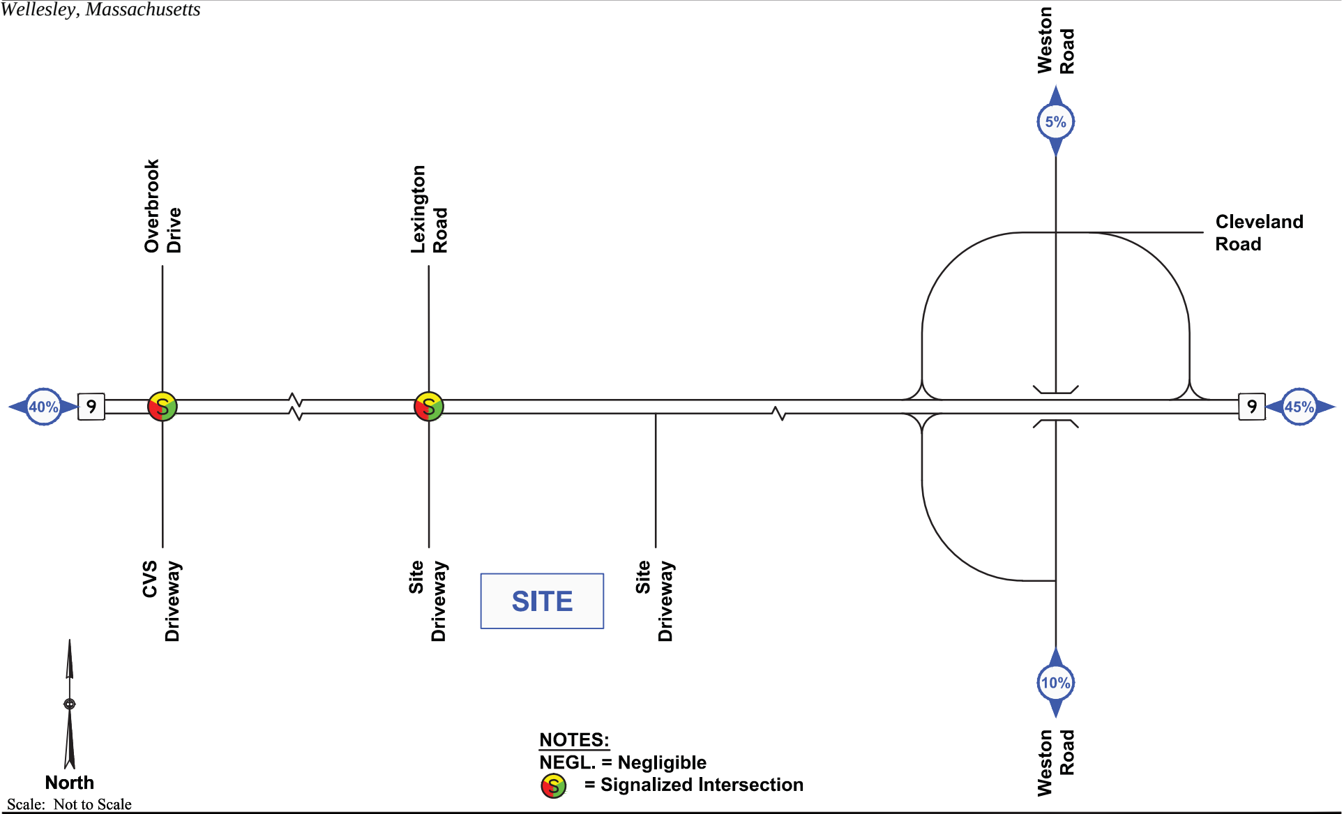
Figure 9 Trip Distribution
